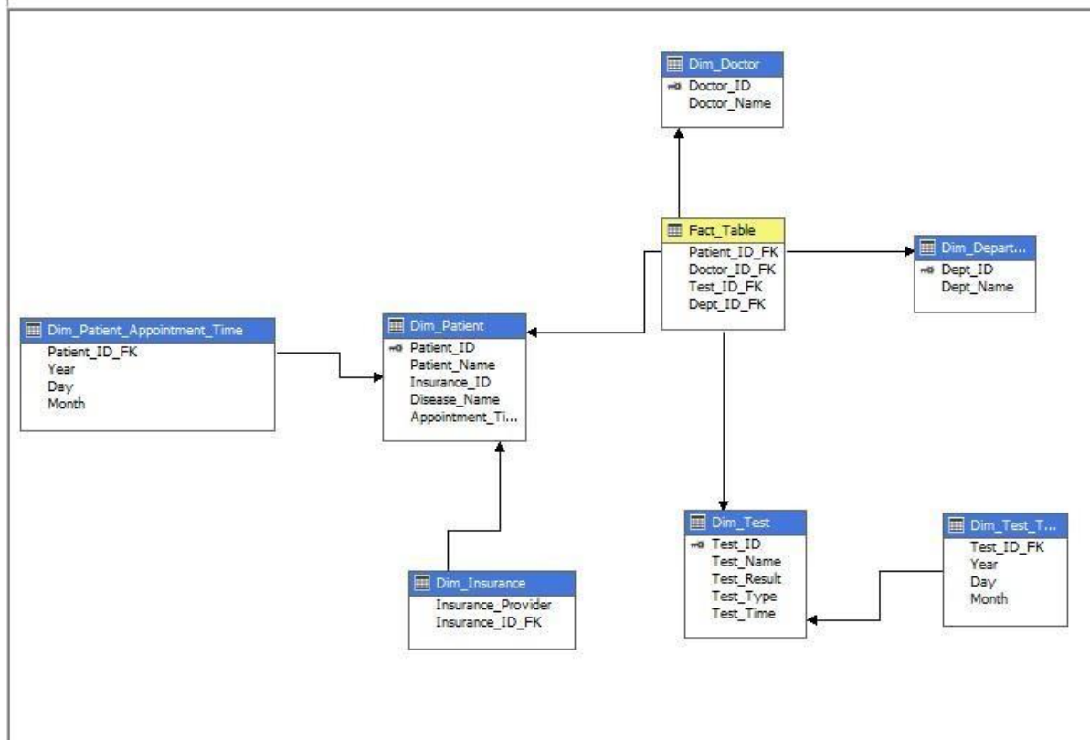
Data Source View
